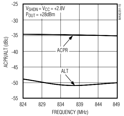
ACPR/ALT vs. FREQUENCY
